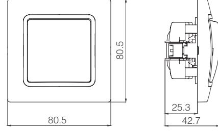
Anahtar
