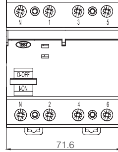
4 Kutuplu (RCCB) 3kA
