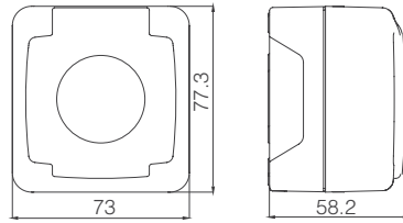
Topraklı Priz
