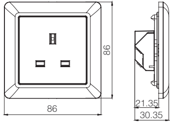
Topraklı Priz
