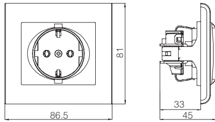
Topraklı Priz
