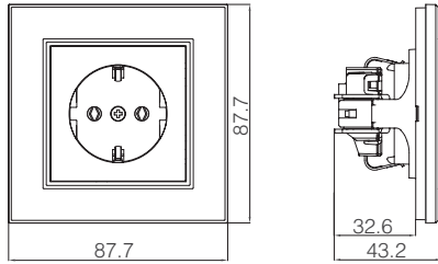
Topraklı Priz
