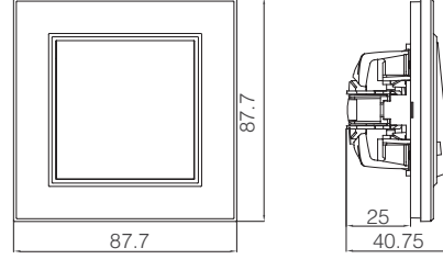
Anahtar
