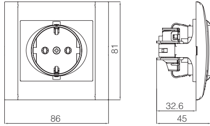
Topraklı Priz
