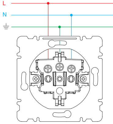
Topraklı Priz
