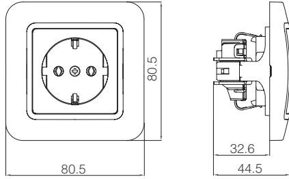
Topraklı Priz
